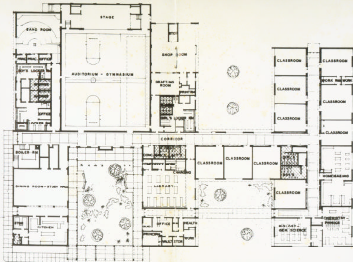
FLOOR PLAN
